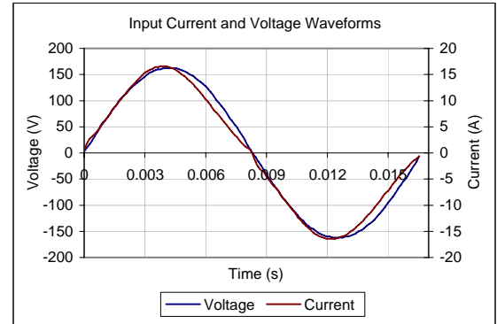
Input AC Current Waveform (ITHD = 6.46%, 50% Load)
