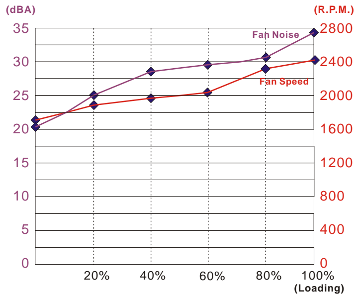
Intelligent Fan speed Controller
